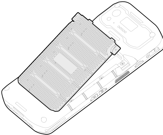
Figure 18 Removing battery – 2
