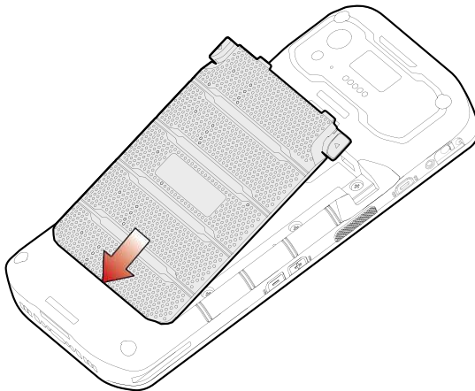
Figure 15 Installing battery – 1
