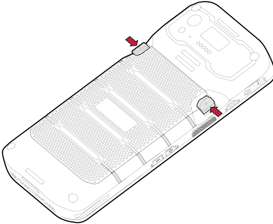
Figure 17 Removing battery – 1
