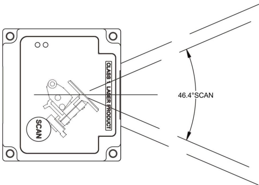
Figure 2-4 Scan angle
