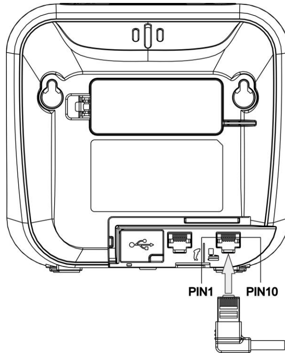
Figure 2-1 Cable connector interface pin-outs
