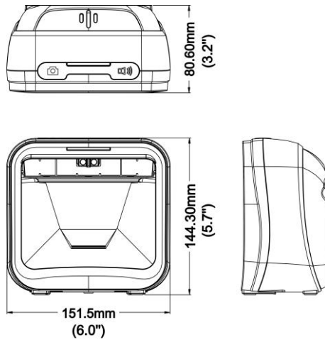
Figure 2-2 Dimensions (without stand)
