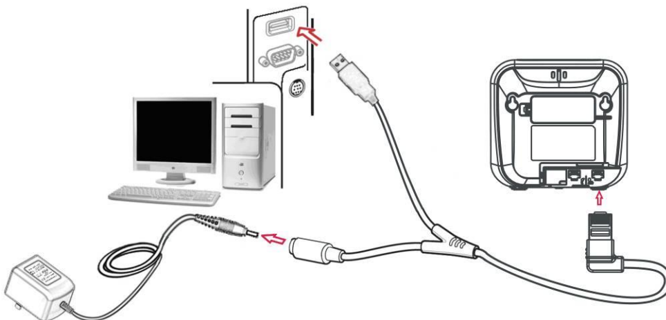
Figure 2-12 Installation of USB cable
