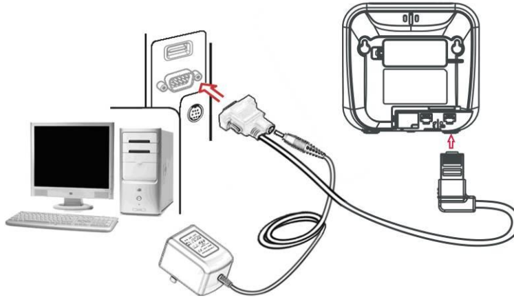
Figure 2-11 Installation of RS232 cable
