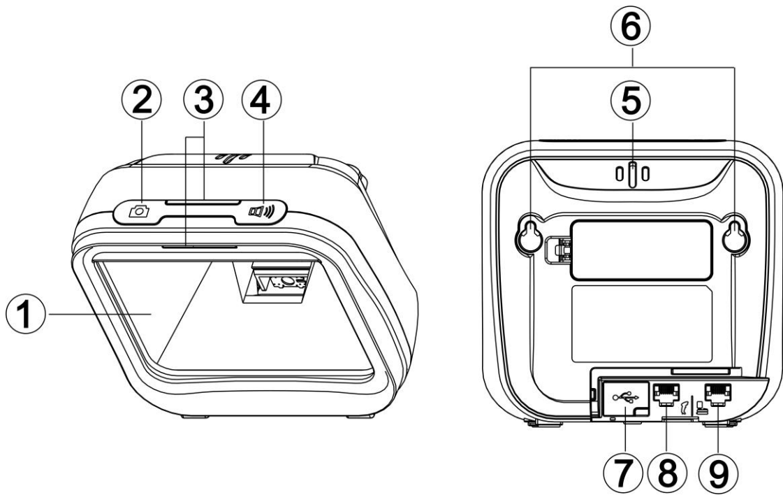
Figure 2-9 Parts of image platform
