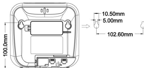
Figure 2-4 Dimensions of hanging holes
