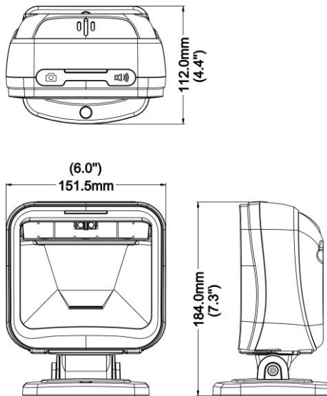
Figure 2-3 Dimensions (with stand)
