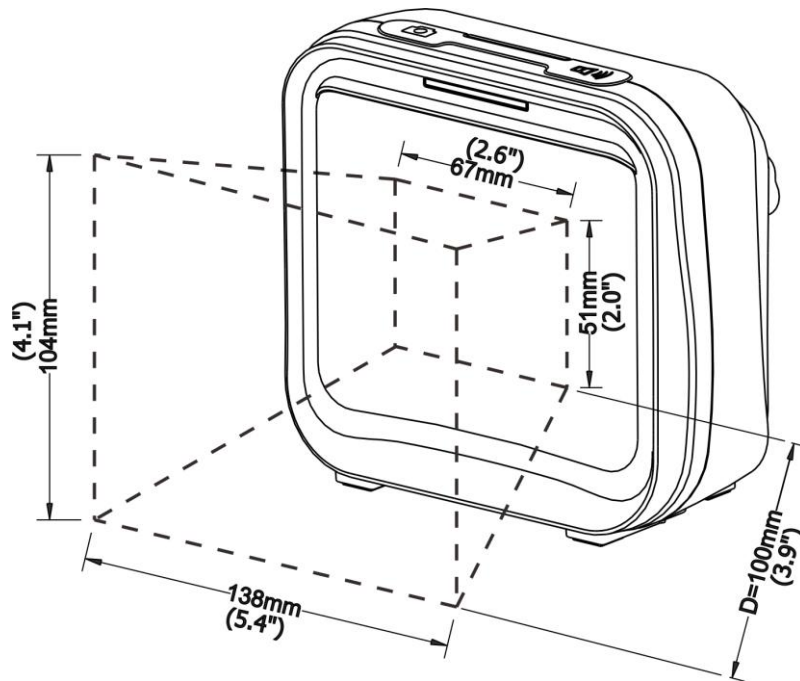
Figure 2-5 Field of view
