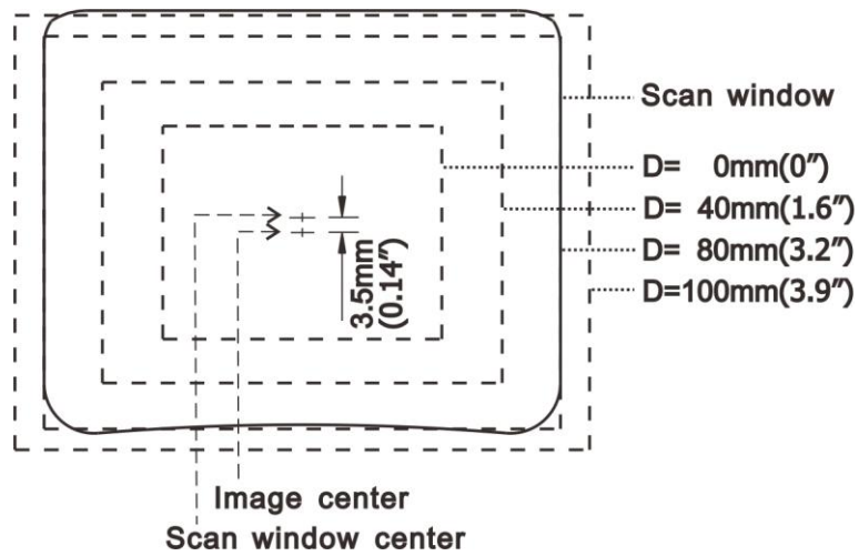
Figure 2-6 Field of view – Front view
