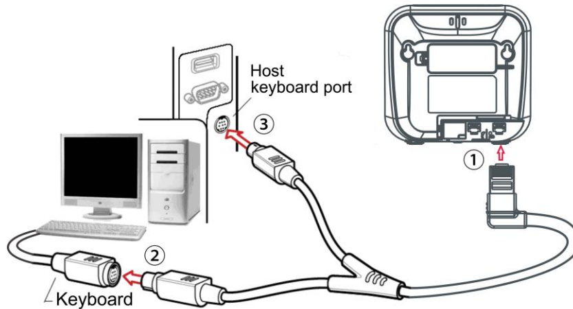
Figure 2-10 Installation of keyboard wedge cable
